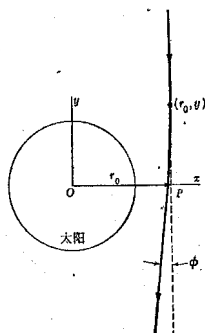
Figure 3. Deflection of photon around the Sun
