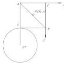
Figure.2 A small ball rolls from A to B
